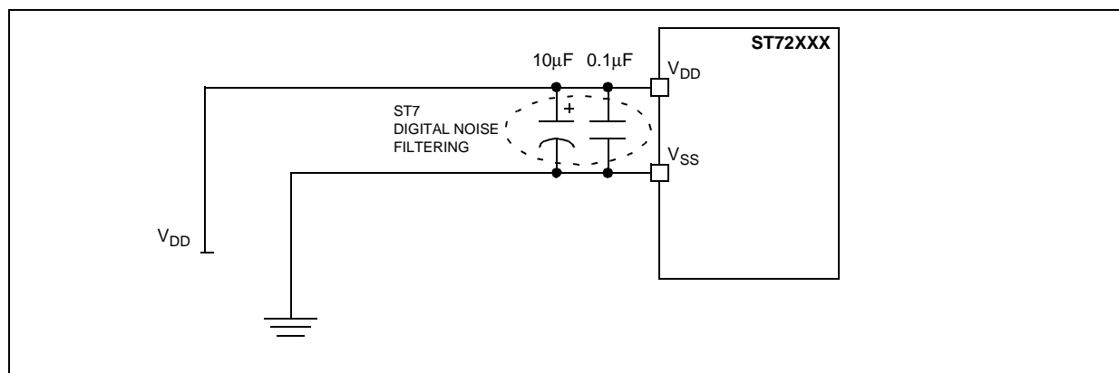
Figure 59. EMC Recommended power supply connection 2)
