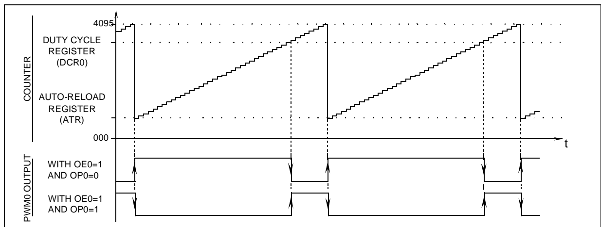
Figure 33. PWM Function
