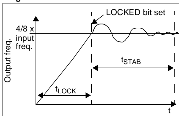
Figure 11. PLL Output Frequency Timing Diagram
