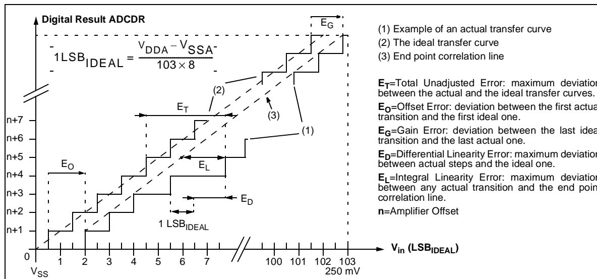
Figure 89. ADC Accuracy Characteristics with Amplifier enabled
