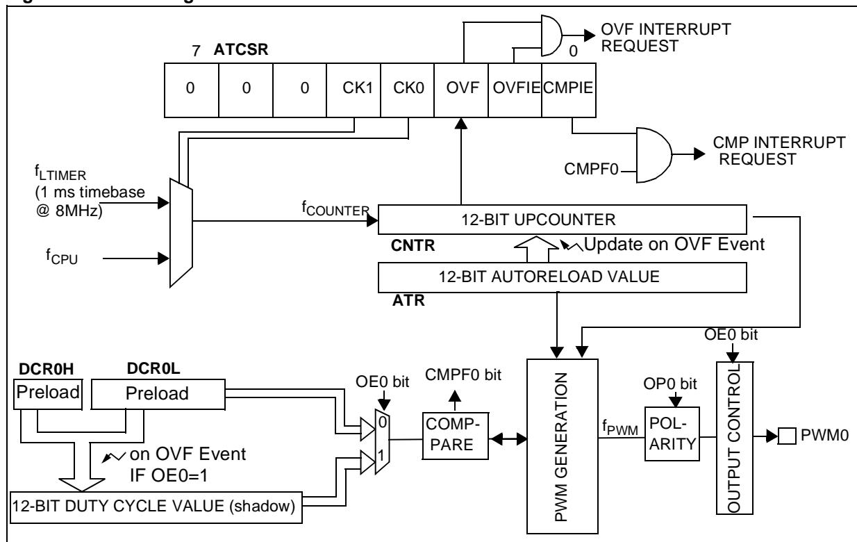
Figure 32. Block Diagram
