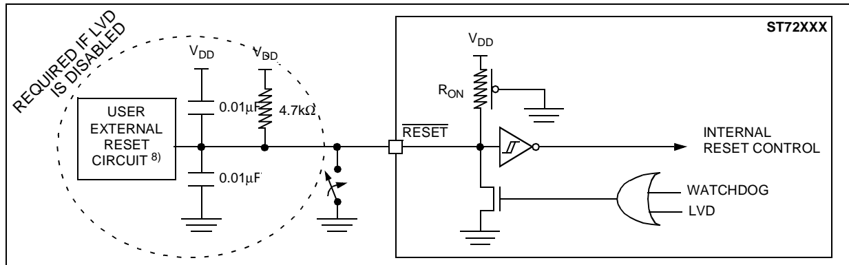
Figure 81. Typical Application with \overline{\text{RESET}} pin 6)7)8)
