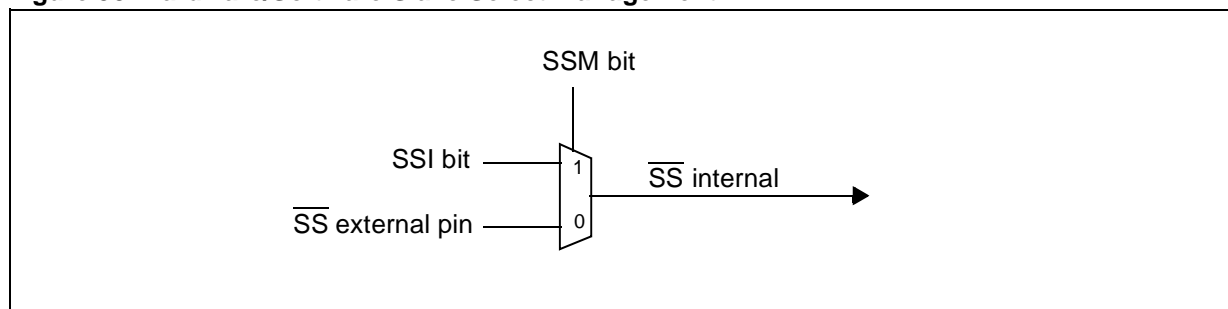
Figure 38. Hardware/Software Slave Select Management
